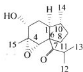
8[7→6]-abeoamorphane, 3 \alpha -hydroxy-4 \alpha ,5 \alpha -epoxy-7-oxo
