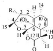
arteannuin D R=OH, n=1
