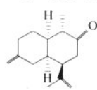
cadina-4(15), 11-dien-9-one
