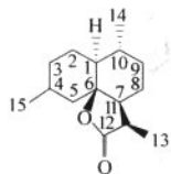
arteannuin K
