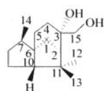
cedrane, 3 \alpha , 15-dihydroxy
