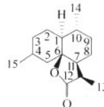
arteannuin B, epi-deoxy
