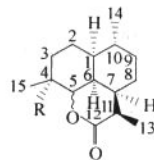
arteannuin F(artemisilactone)
