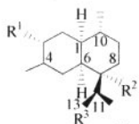
cadina-4-ene, 3 \alpha , 7 \alpha -dihydroxy
