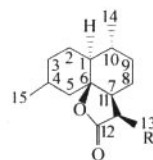
artemisia dihydroxycadinolide
