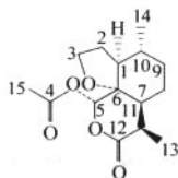
arteannuin G
