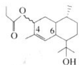
cadia-4-en-11-ol, 3-iso-butyryl
