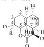
arteannuin I
